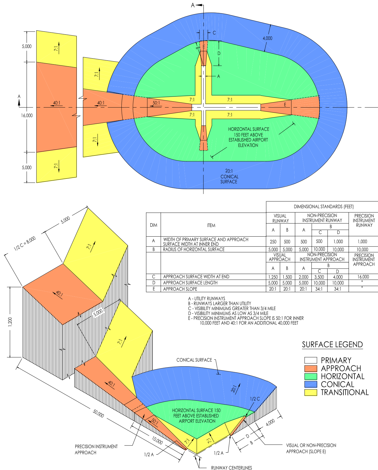
ISOMETRIC VIEW OF SECTION A-A
