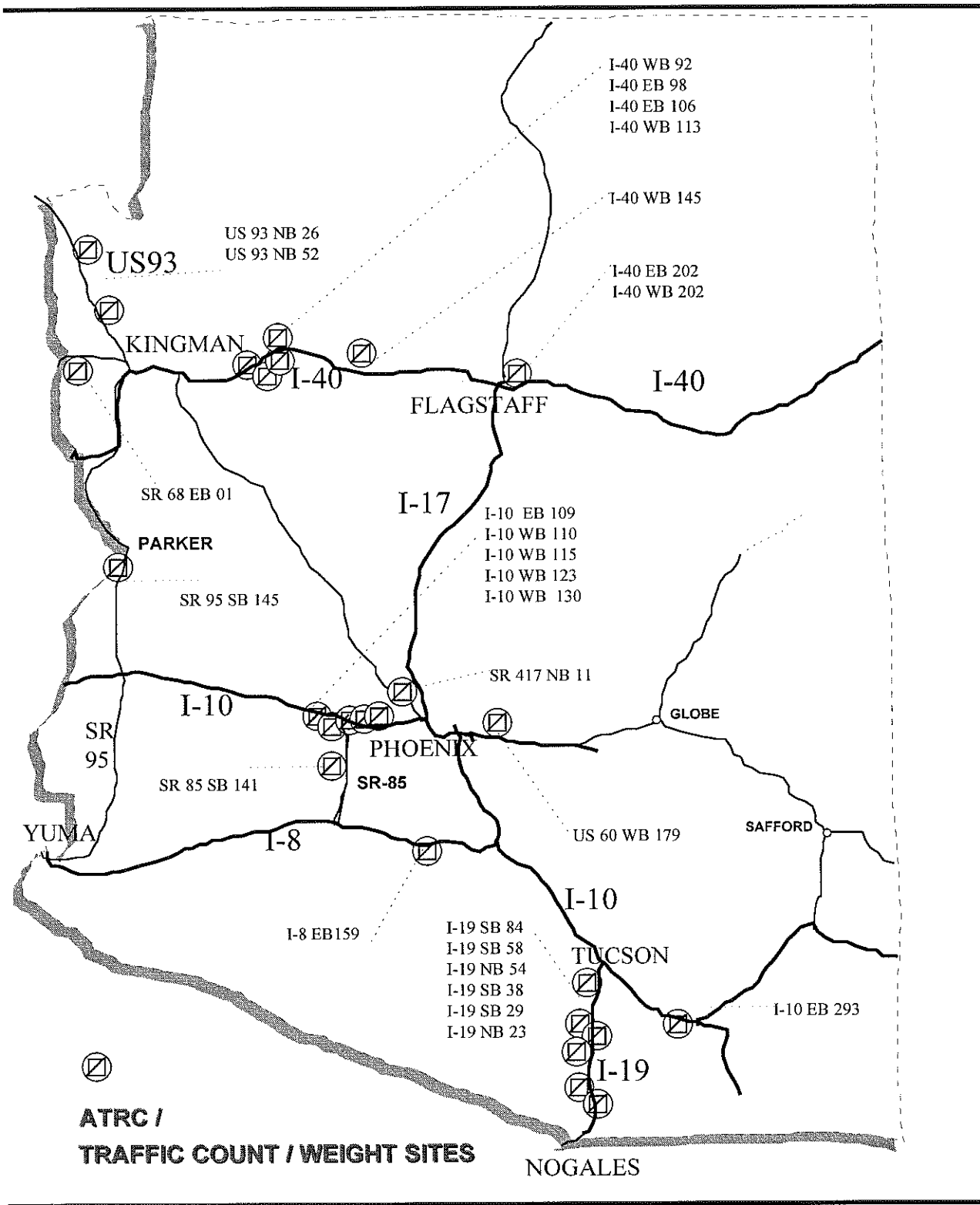
Figure 1 Arizona LTTP Traffic Data Collection Sites as of June, 1996
