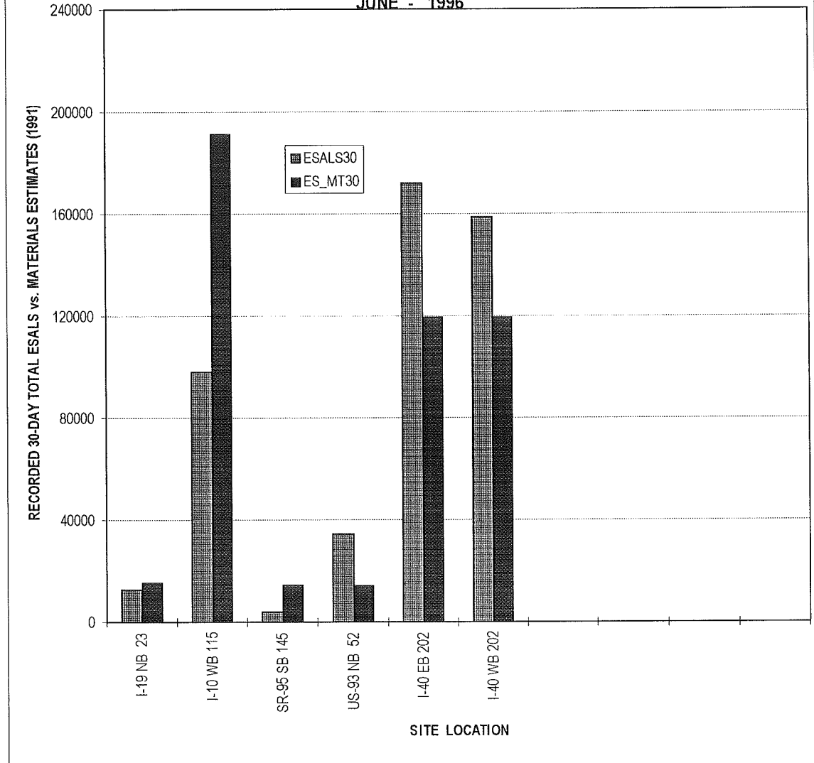
30-DAY TOTAL ESALS (18-KIP) CHART FOR JUNE - 1996
