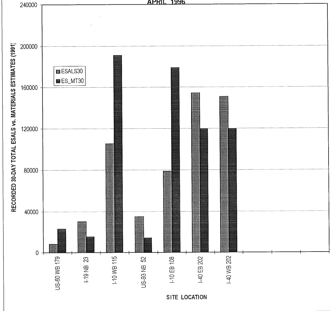
30-DAY TOTAL ESALS (18-KIP) CHART FOR APRIL 1996
