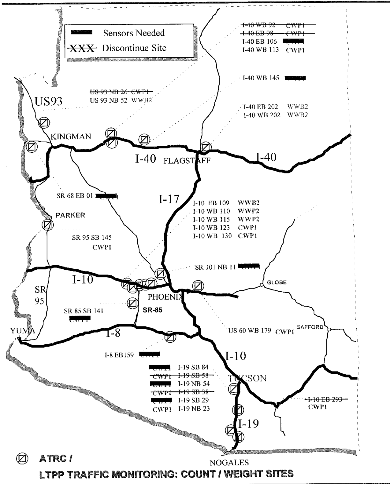
Figure 2 Status of Arizona LTPP Traffic Data Collection Sites as of June, 1996
