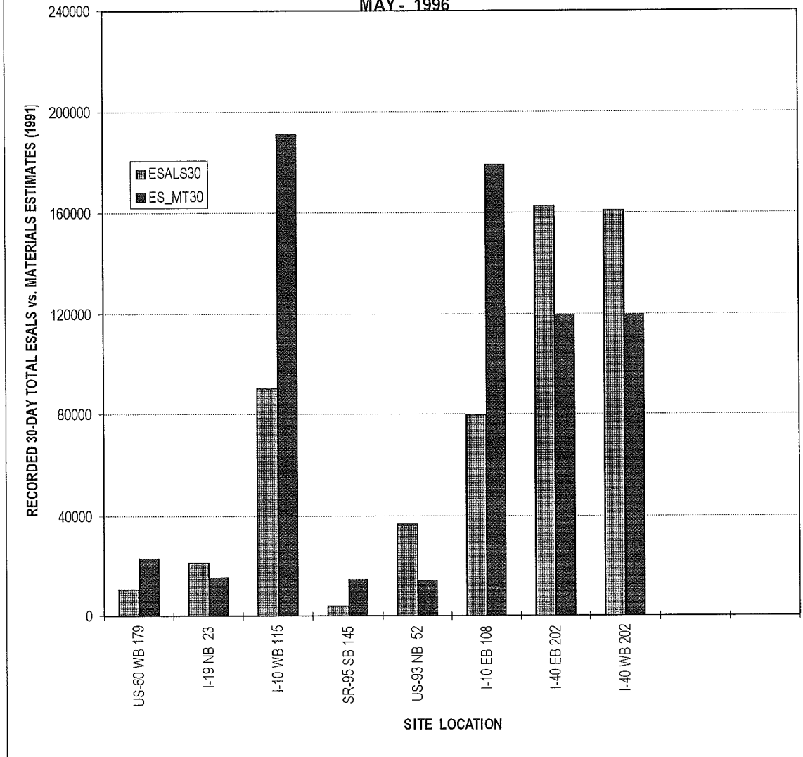
30-DAY TOTAL ESALS (18-KIP) CHART FOR MAY - 1996
