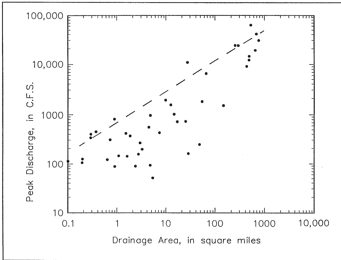
FIGURE 10-19 Q_{100} DATA POINTS AND 100-YEAR PEAK DISCHARGE RELATION FOR R11
