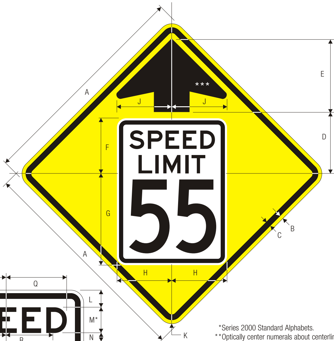
W3-5 SPEED REDUCTION
