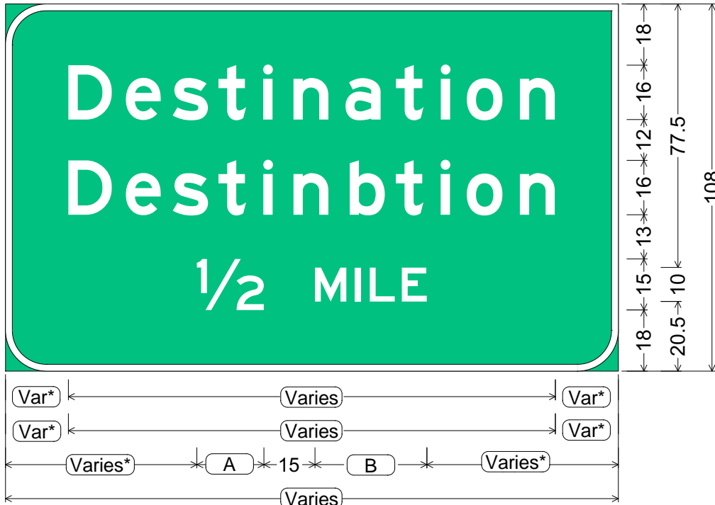
E1-102b; 12.00" Radius, 2.00" Border, White on Green; "Destination" E; "Destinbtion" E; "1/2" E; "MILE" E;
